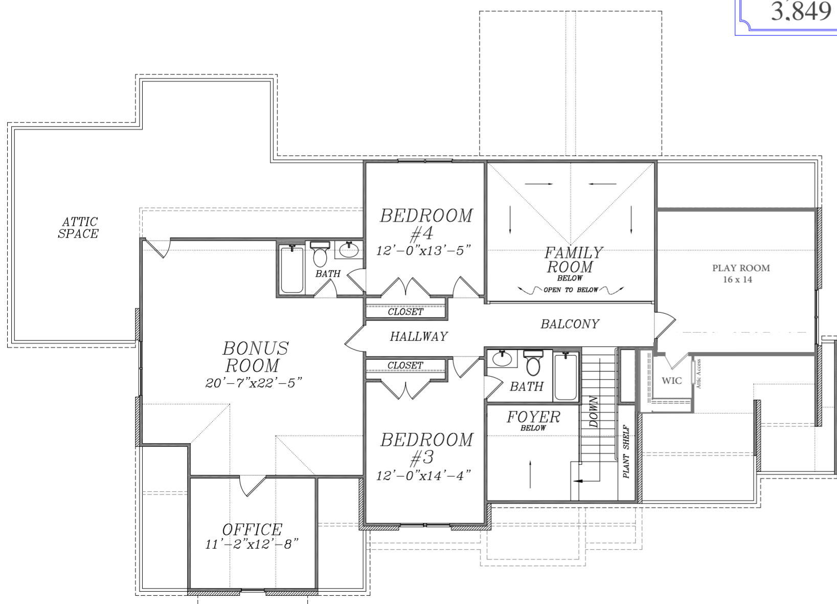
SECOND FLOOR 9'-0" CEILING HEIGHT
