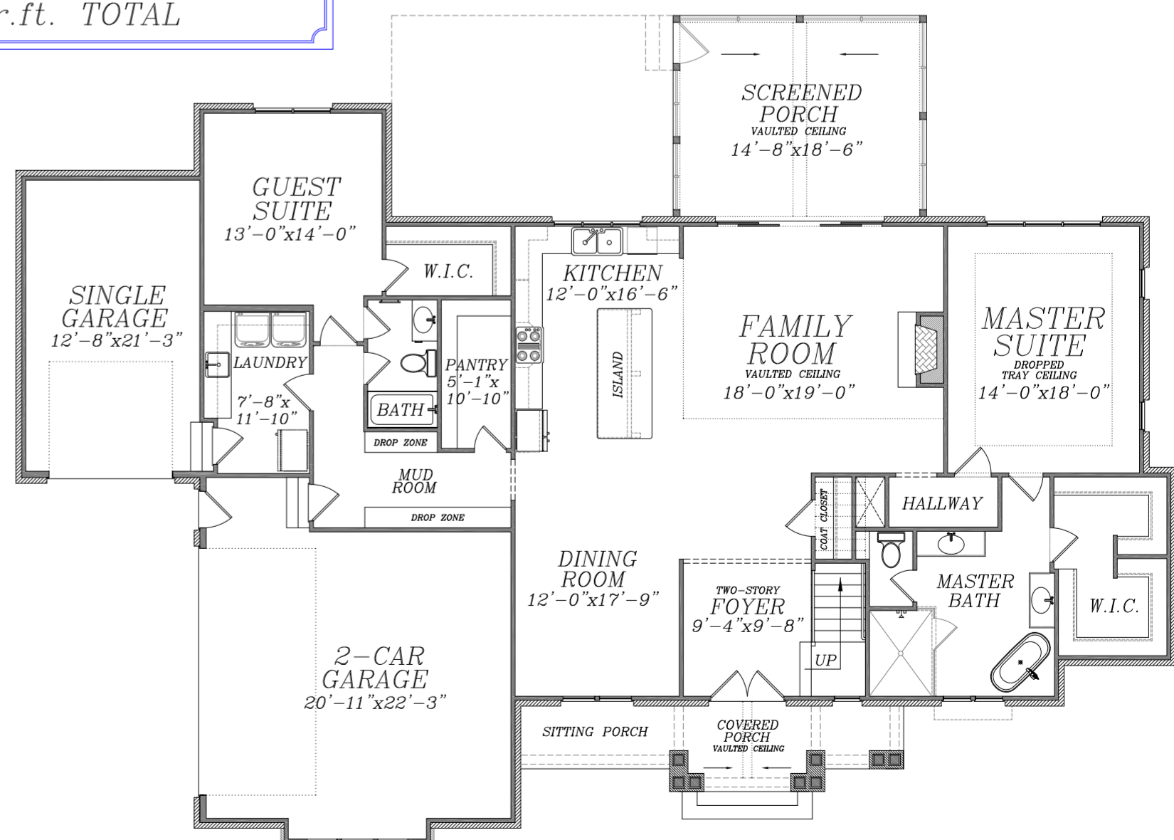
FIRST FLOOR 10'-0" CEILING HEIGHT
